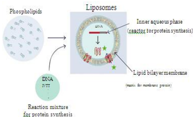
Figure 4: Liposomes as a platform for in vitro protein synthesis. The reaction mixture for protein synthesis constitutes an inner aqueous phase of the liposome, in which protein is synthesized from a DNA. Membrane protein synthesized inside liposome can be embedded into a lipid bilayer membrane.
