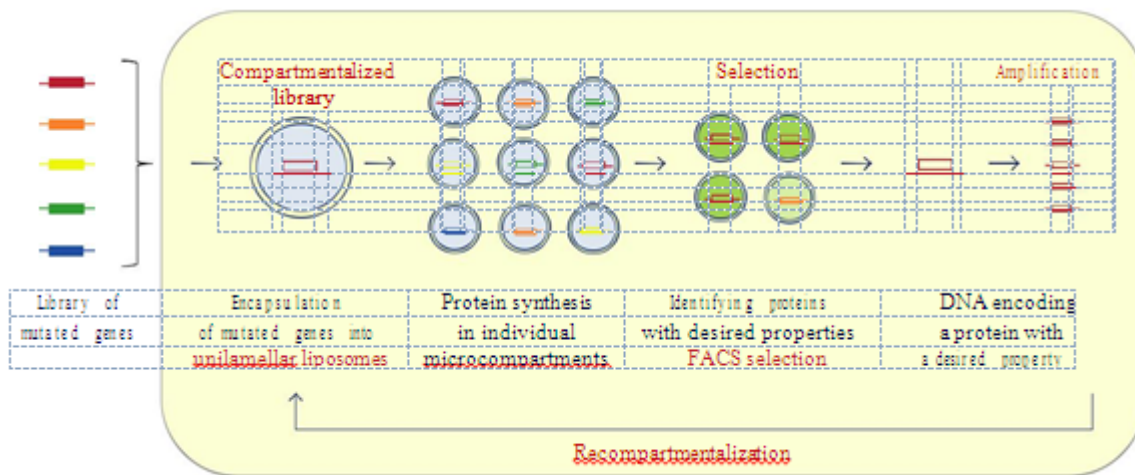
Figure 6: the Flowchart for protein screening using liposome-based IVC. Library of mutated genes is compartmentalized with the PURE system and other reagents into the liposome. Each protein variant is synthesized from a single copy of the gene in each liposome. Liposomes encapsulating the gene of interest are screened using a FACS. DNA extracted from the liposomes is amplified to be transferred to the next round of gene screening.
