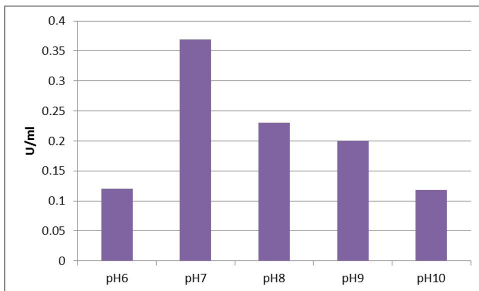
FIG 3: Effect of pH on production of catechol 1,2-dioxygenase.
