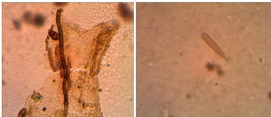
Algal filament with Curvularia
