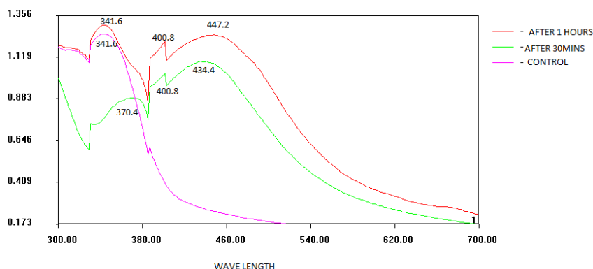
Fig. 3 - UV-Vis spectra of leaf extract of NA (control) and silver nanoparticles prepared thereof after 30 mins and 1 hour.
