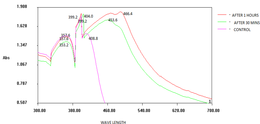
Fig. 2 - UV-Vis spectra of leaf extract of JA (control) and silver nanoparticles prepared thereof after 30 mins and 1 hour.
