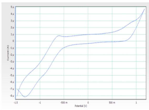
Figure- 6c CV curve of Ni-PMA.
