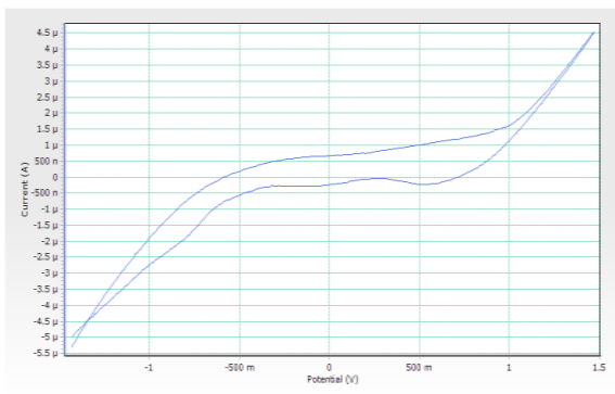
Figure-5a CV curve of Mn-PMA complex. Figure-5b CV curve of Co-PMA complex.
