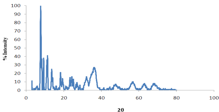
Fig:3: \text{FeZn}(\text{SB})_2(\text{H}_2\text{O})_2 .
