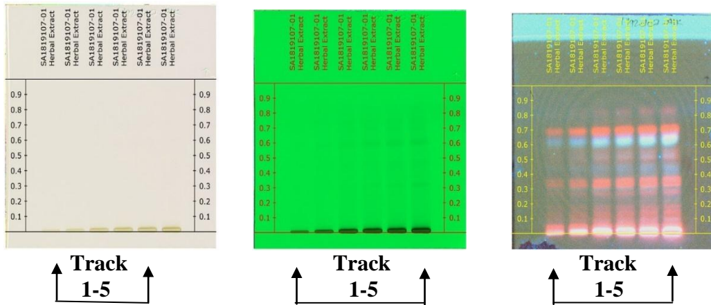
Chromatogram at visible Chromatogram at 254 nm Chromatogram at 366 nm Track 1-5: Methanol extract of Ailanthus excelsa leaves.
